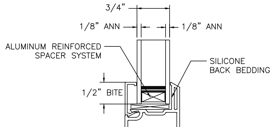
GLAZING DETAIL
