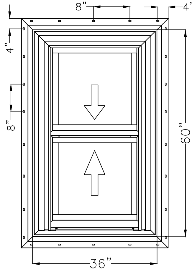
1650 PVC DH WINDOW – FIN INSTALLATION MAXIMUM SIZE 30" X 60" DESIGN PRESSURE +/- 50 PSF NON-IMPACT
